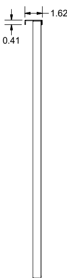
Pull tab placement on slab door.
