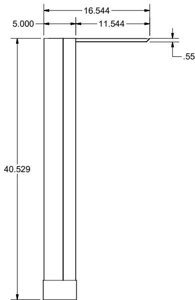
OCPSxx (NO electrical cutout)
