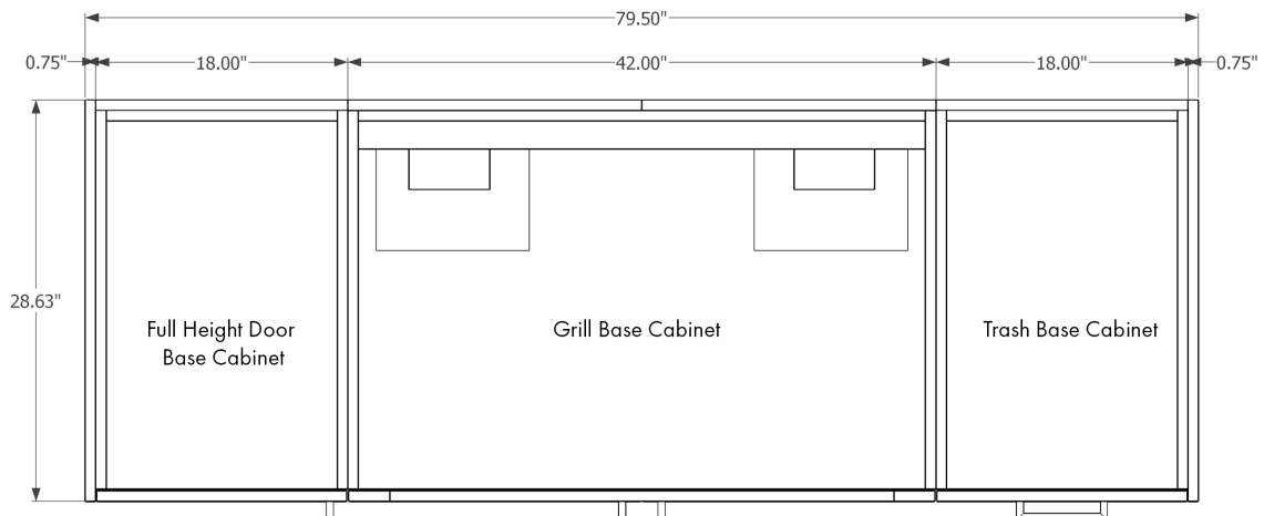
Displayed with Finished Side & Back Panels
